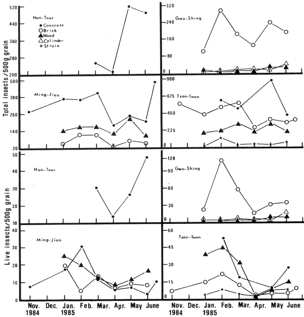
圖二 臺灣中部地區不同倉型之稻穀倉中積穀害蟲密度變化。 Fig. 2. Population changes of stored products insect pests in different type of bins in central Taiwan from November 1984 to June 1985.
