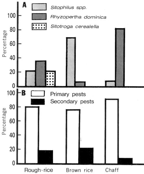
圖一 初級及次級害蟲在稻穀、糙米及粗糠中之分布情形。(A)初級害蟲種類(B)初級及次級害蟲。 Fig. 1. Percentage of primary and secondary pests in stored rough rice, brown rice and chaff in Taiwan. (A) Species of primary pests, (B) Primary and secondary pests.
